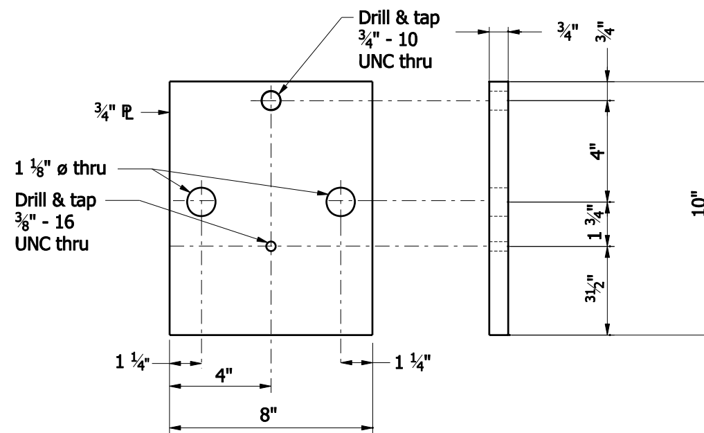
BASE PLATE
