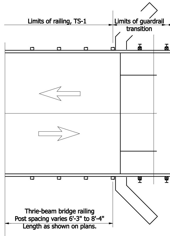
PLAN VIEW
