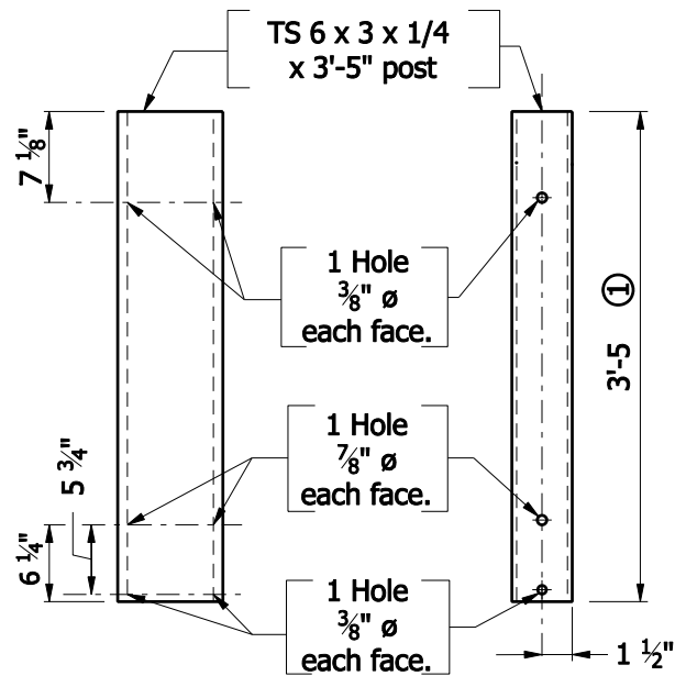
SECTION BRIDGE STEEL POST DETAIL
