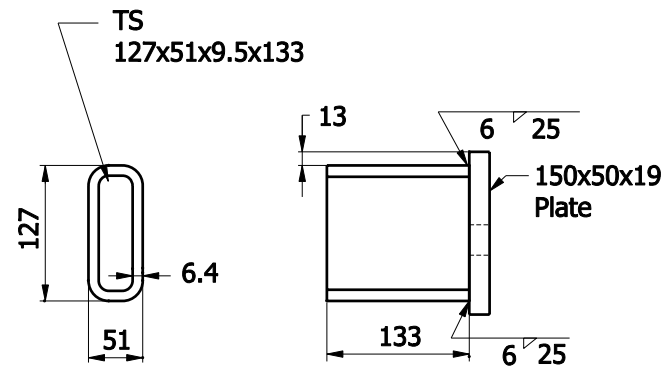
STEEL TUBE SPACER ASSEMBLY
