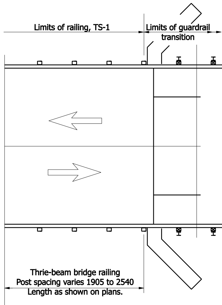
PLAN VIEW
